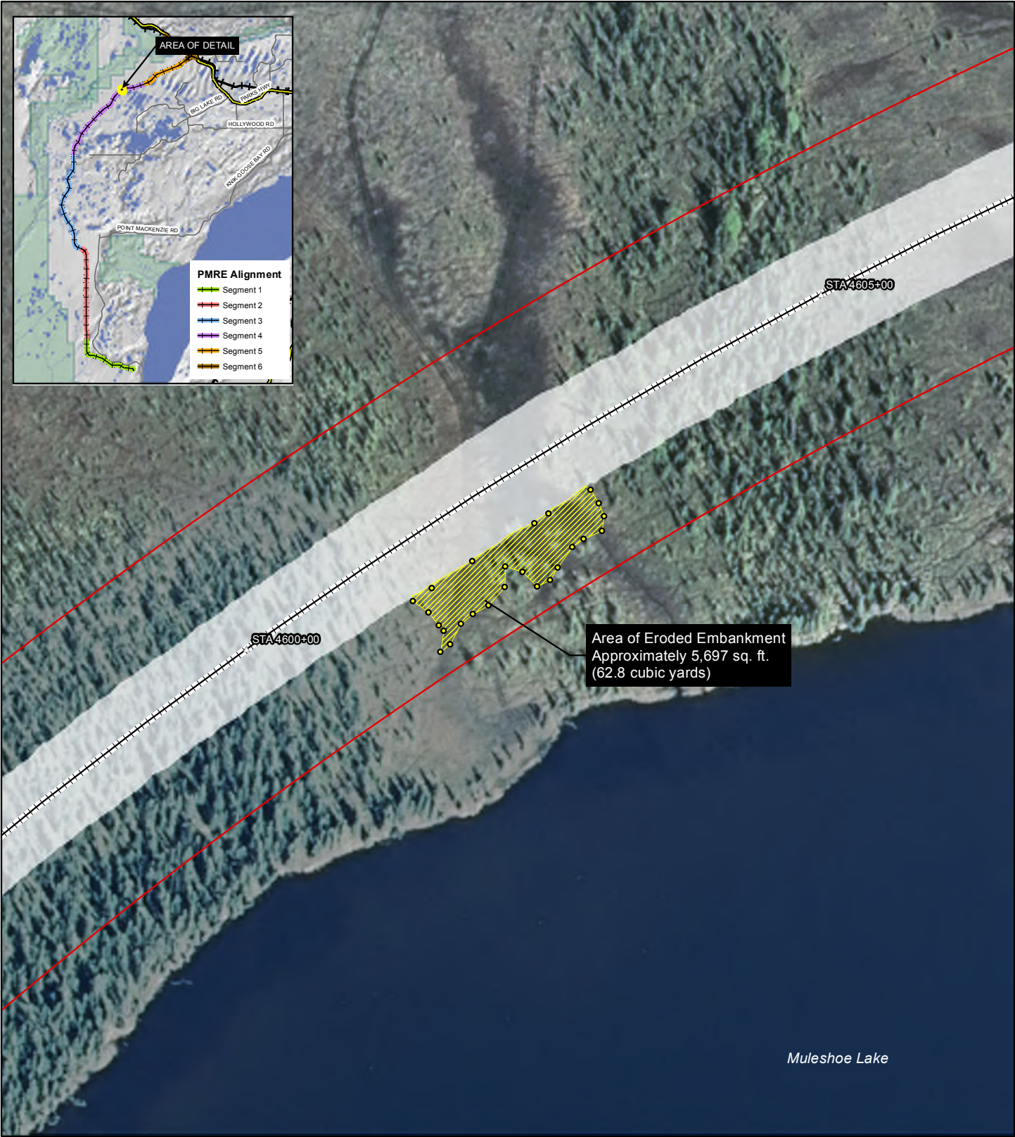
Figure 22: Map of washout fill area on Segment 4
