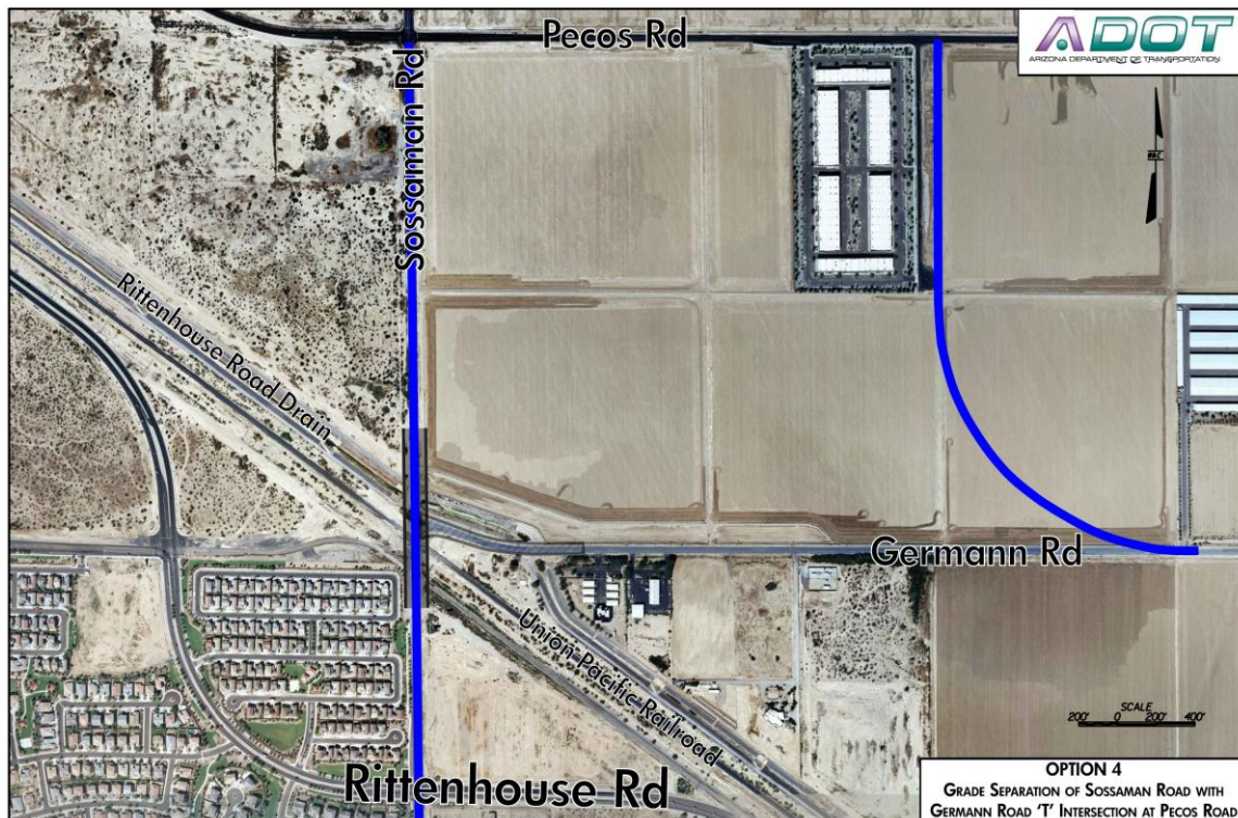
FIGURE 8-6 NETWORK CONNECTIVITY OPTION 4
