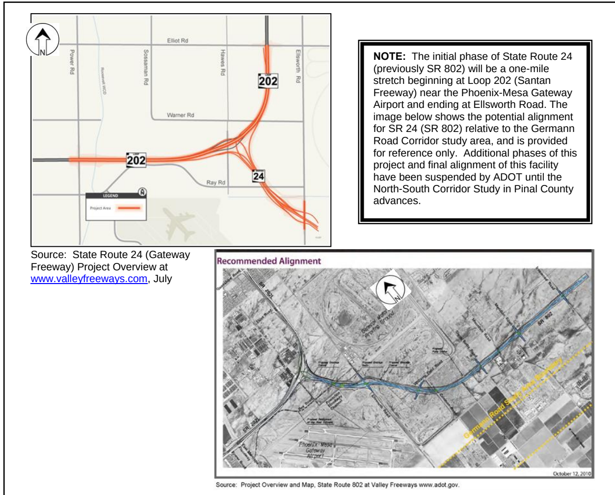
FIGURE 7-1 RECOMMENDED ALIGNMENT OF SR 24 (FORMERLY SR 802): LOOP 202 TO IRONWOOD ROAD
