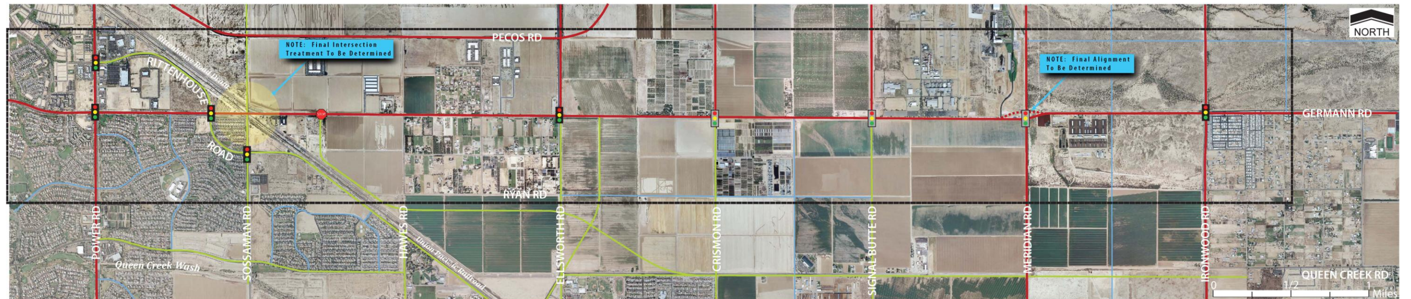
FIGURE 8-1 RECOMMENDED ALIGNMENT OF GERMANN ROAD: POWER ROAD TO IRONWOOD ROAD
