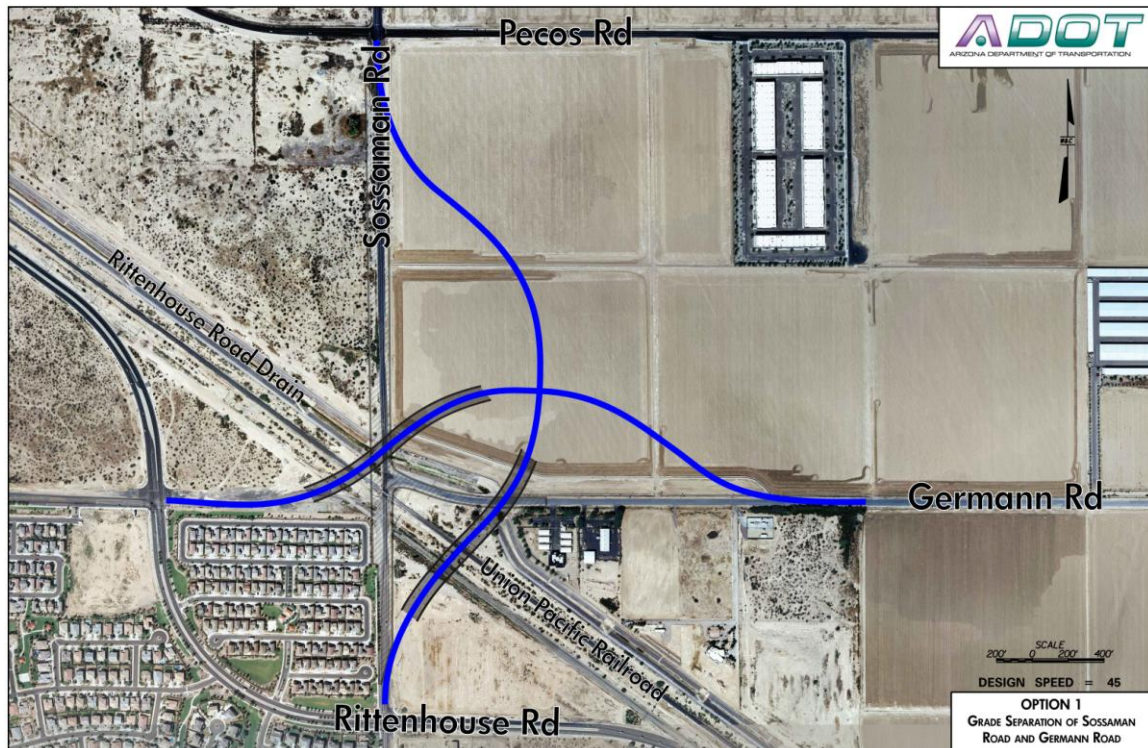
FIGURE 8-3 NETWORK CONNECTIVITY OPTION 1
