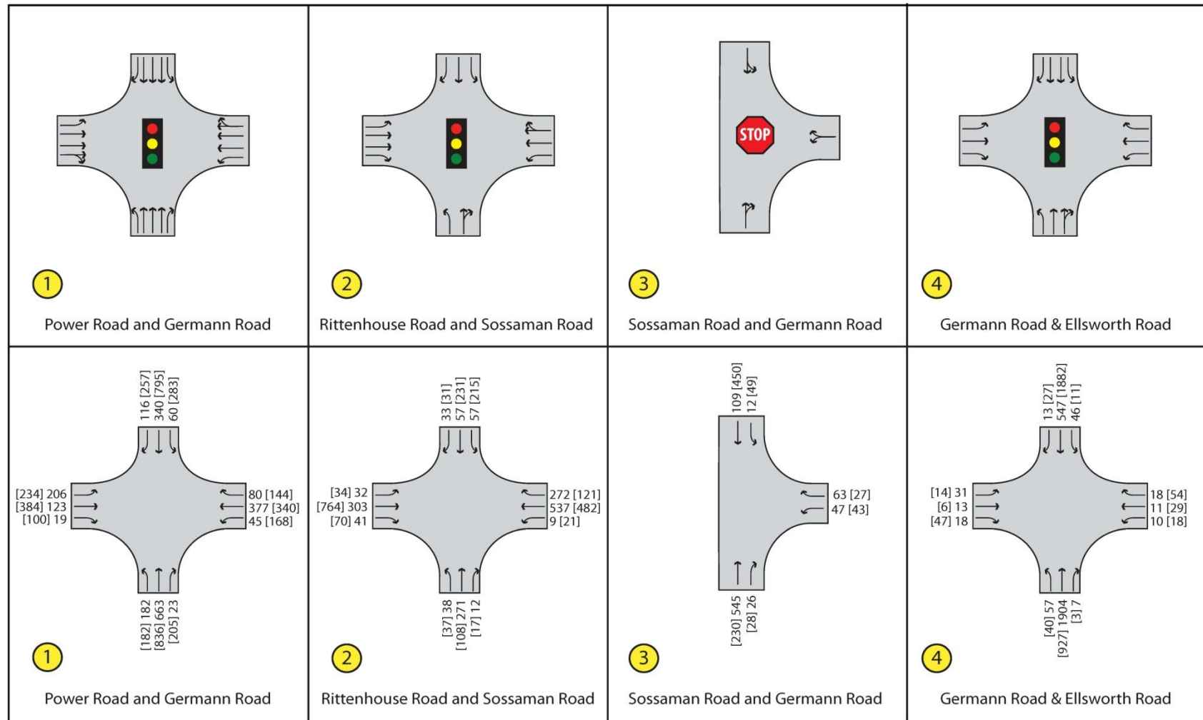
FIGURE 3-2 EXISTING INTERSECTION GEOMETRICS AND TURNING-MOVEMENT VOLUMES
