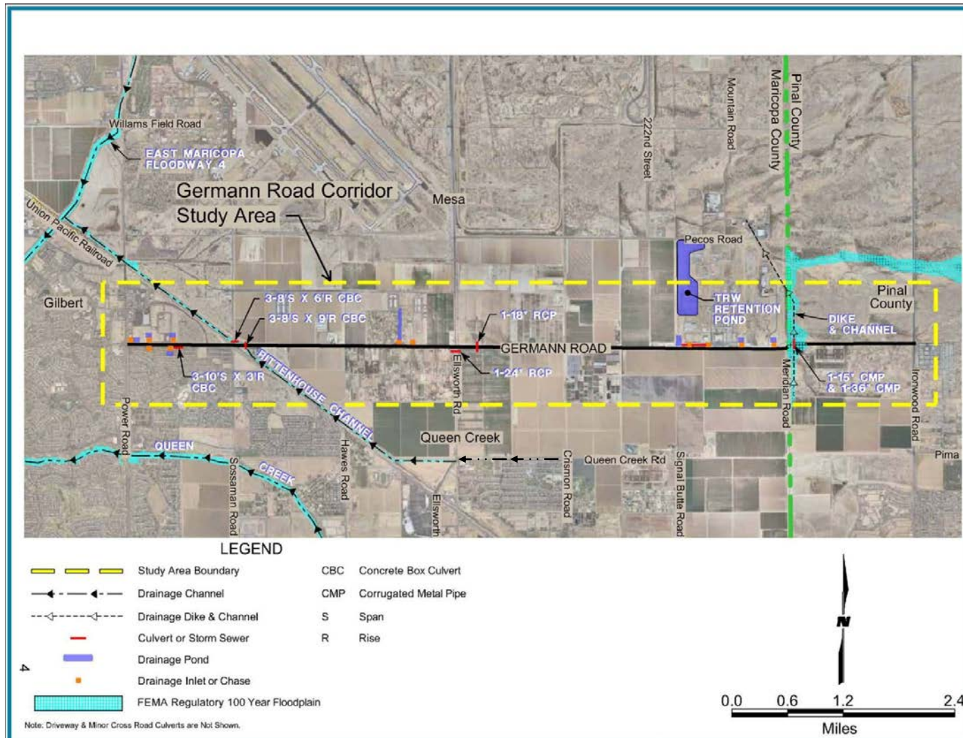
FIGURE 5-2 EXISTING GERMANN ROAD CORRIDOR DRAINAGE IMPROVEMENTS
