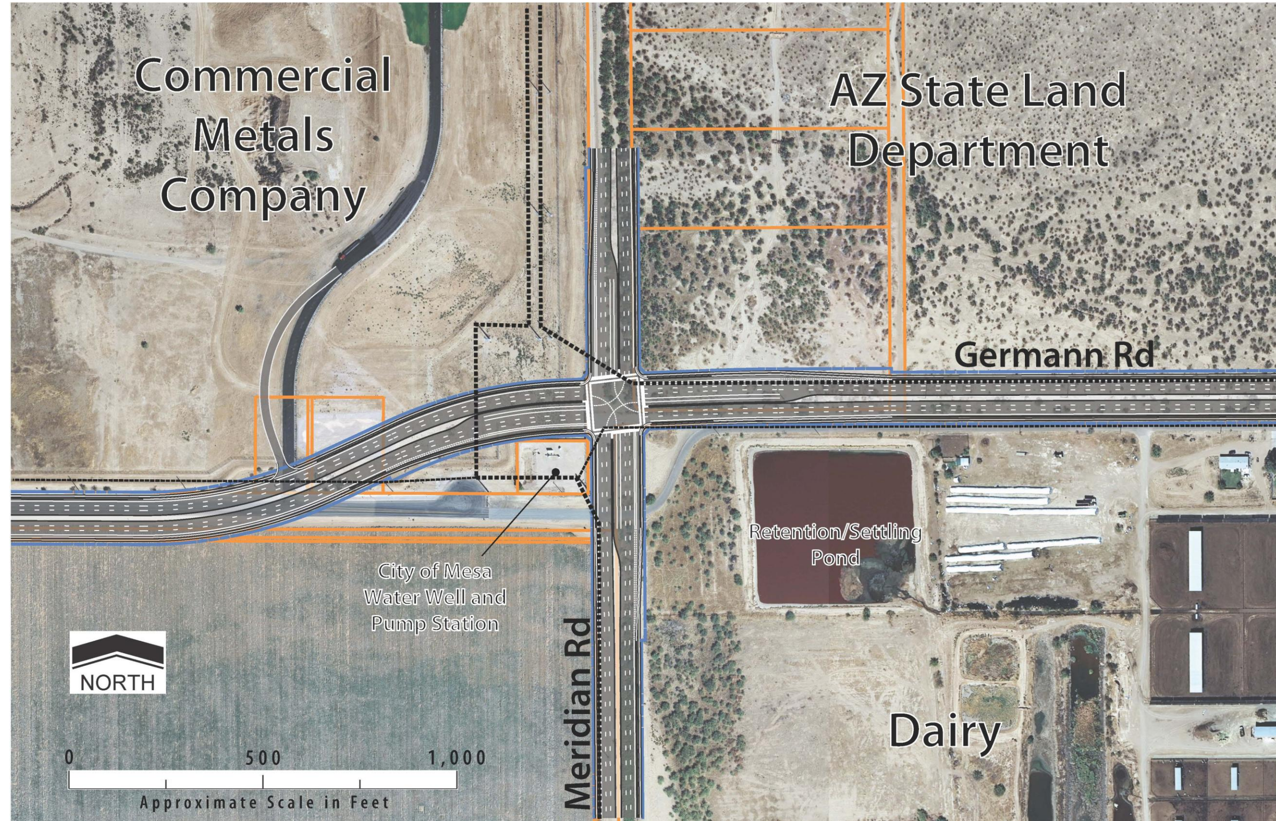
FIGURE 8-12 GERMANN/MERIDIAN INTERSECTION ALTERNATIVE 2 – NORTHERN DIVERSION
