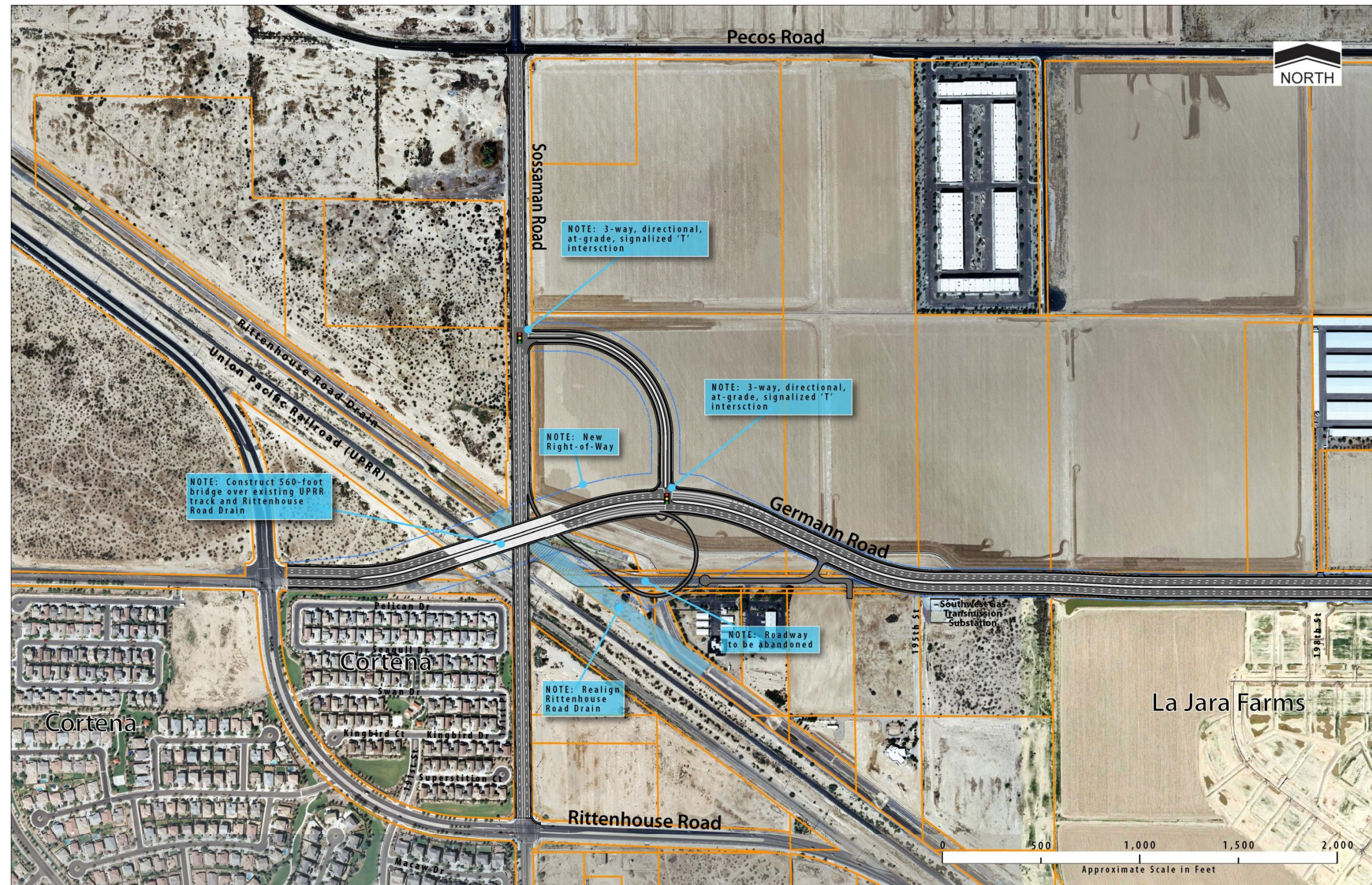
FIGURE 8-10 ALTERNATIVE C – GRADE SEPARATION OF GERMANN ROAD ONLY WITH RAMP TO NORTHBOUND SOSSAMAN ROAD AND CONNECTOR TO SOSSAMAN ROAD
