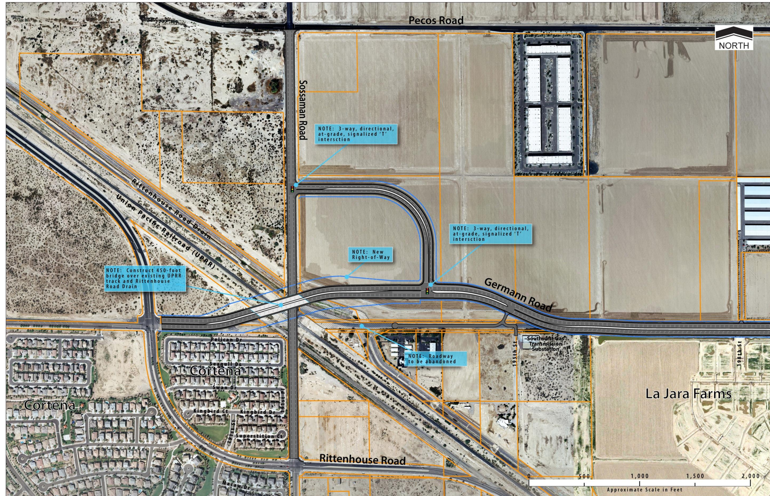
FIGURE 8-9 ALTERNATIVE B – GRADE SEPARATION OF GERMANN ROAD ONLY WITH ACCESS TO SOSSAMAN ROAD
