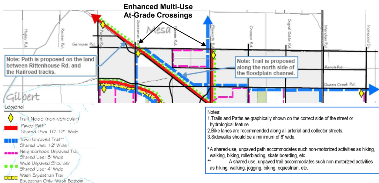
FIGURE 7-4 QUEEN CREEK TRAILS AND PATHS PLAN
