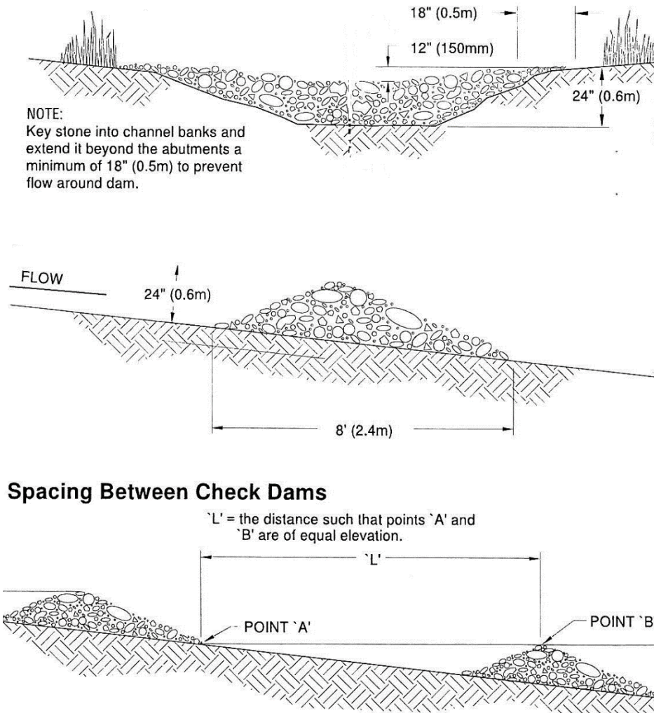
Figure 9. Schematic of check dam specifications.
