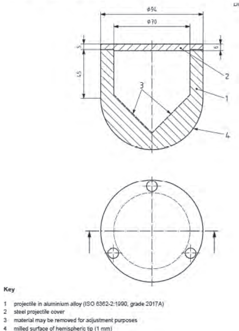
Figure 1 to paragraph (b)(2)(i)(D) - Large Object Glazing Test Projectile
