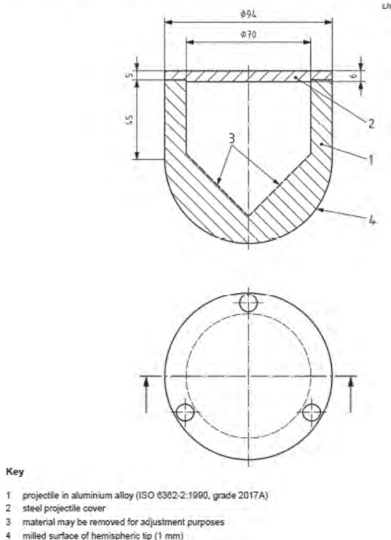
Figure 6 to paragraph (b)(2)(i)(D) - Large Object Glazing Test Projectile
