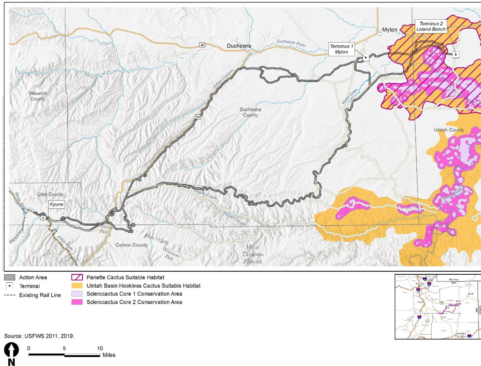
Figure 4-11. Pariette Cactus and Uinta Basin Hookless Cactus Suitable Habitat in the Action Areas
